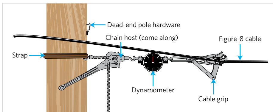
Figure 6: Tensioning setup
